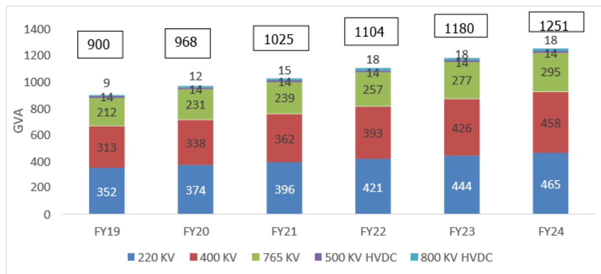
Chart 40: Transformation Capacity (220 kV & Above)
