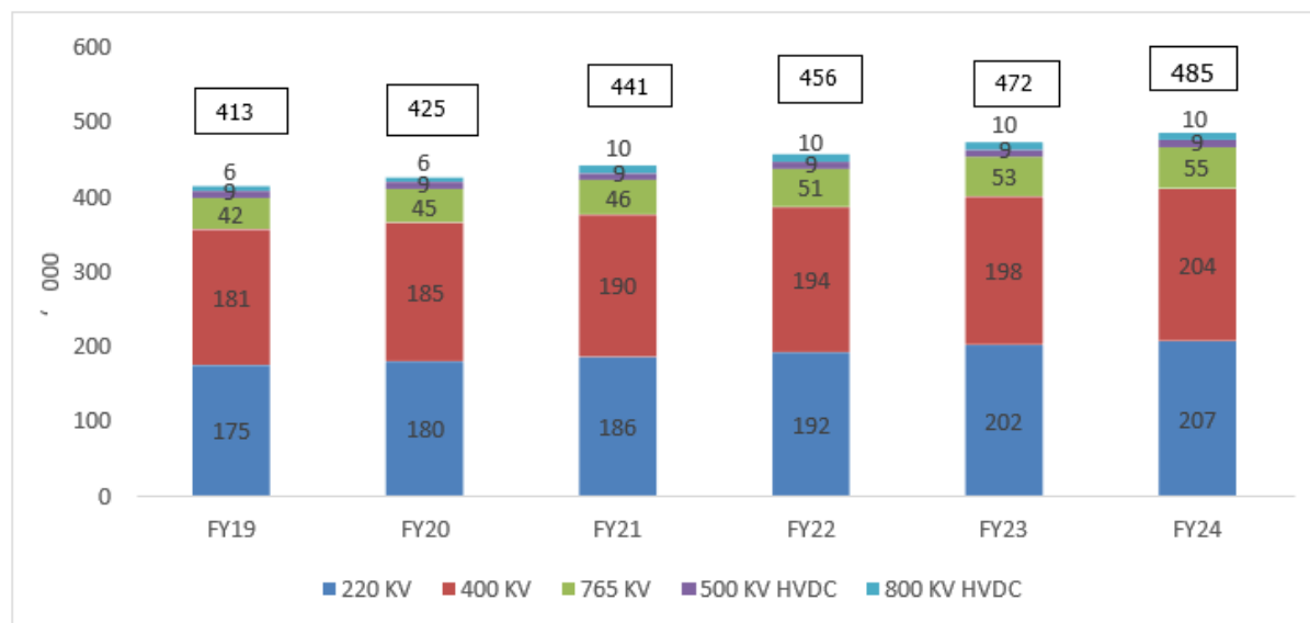
Chart 41: Transmission Line Network (220 kV & Above)
